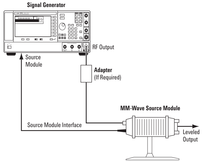
Figure 3-4. External Millimeter- wave source module leveling with an Option 1EA signal generator.
