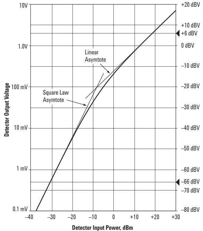
Figure 3-2. Typical diode detector response at 25° C.
