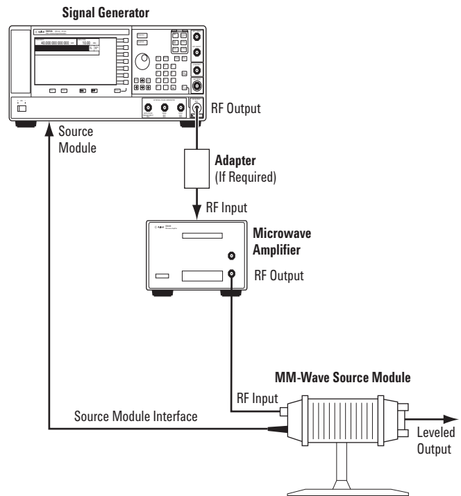
Figure 3-3. External Millimeter-wave source module leveling for a signal generator without Option 1EA.
