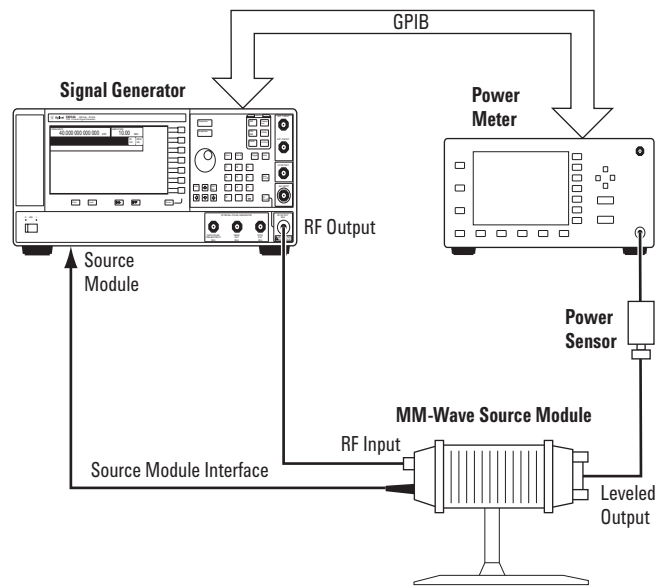
Figure 3-7. User flatness with mm-wave source module and option 1EA signal generator.
