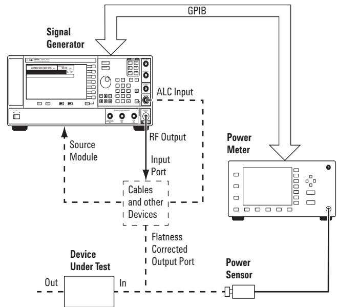
Figure 3-5. User Flatness Correction Equipment Setup.
