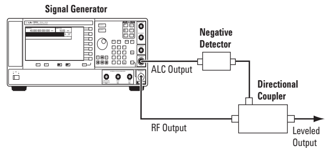
Figure 3-1. External detector leveling with a directional coupler.
